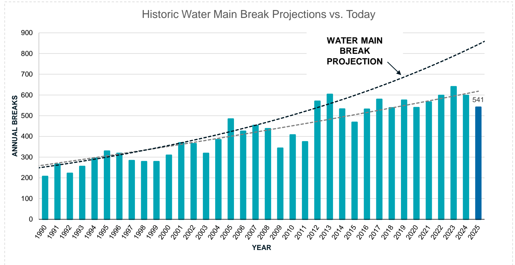
Analysis of historical water main break
