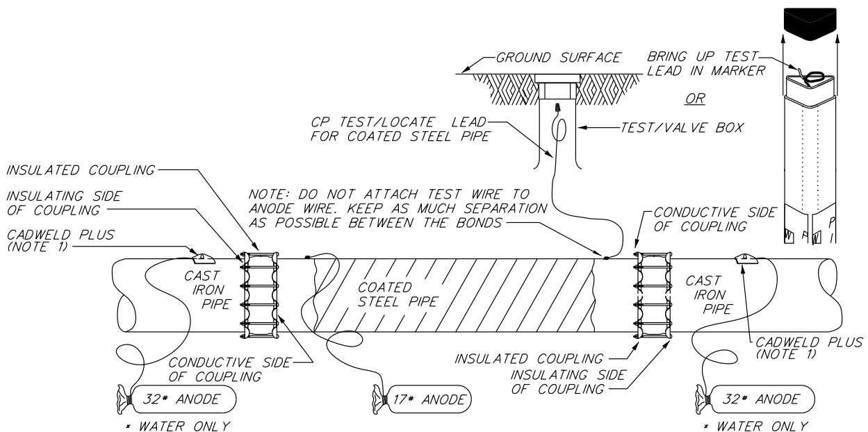
FIG 10 - COATED STEEL TO CAST IRON CONNECTION DETAIL
