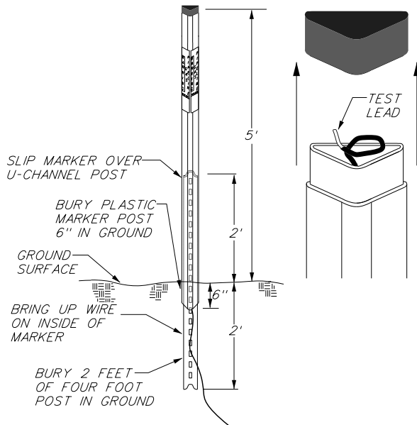
FIG 4 - MARKER POST DETAIL WHEN ONLY ONE WIRE IS USED
