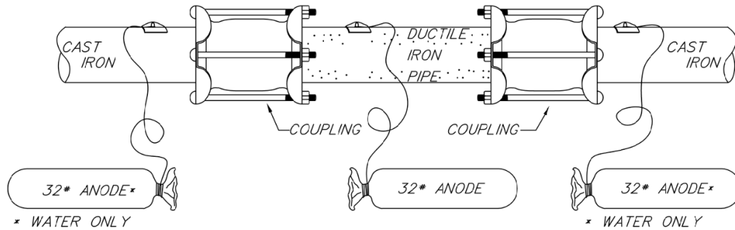
FIG 11 - REPLACING SECTION OF CAST IRON WITH DUCTILE IRON USING STEEL COUPLINGS
