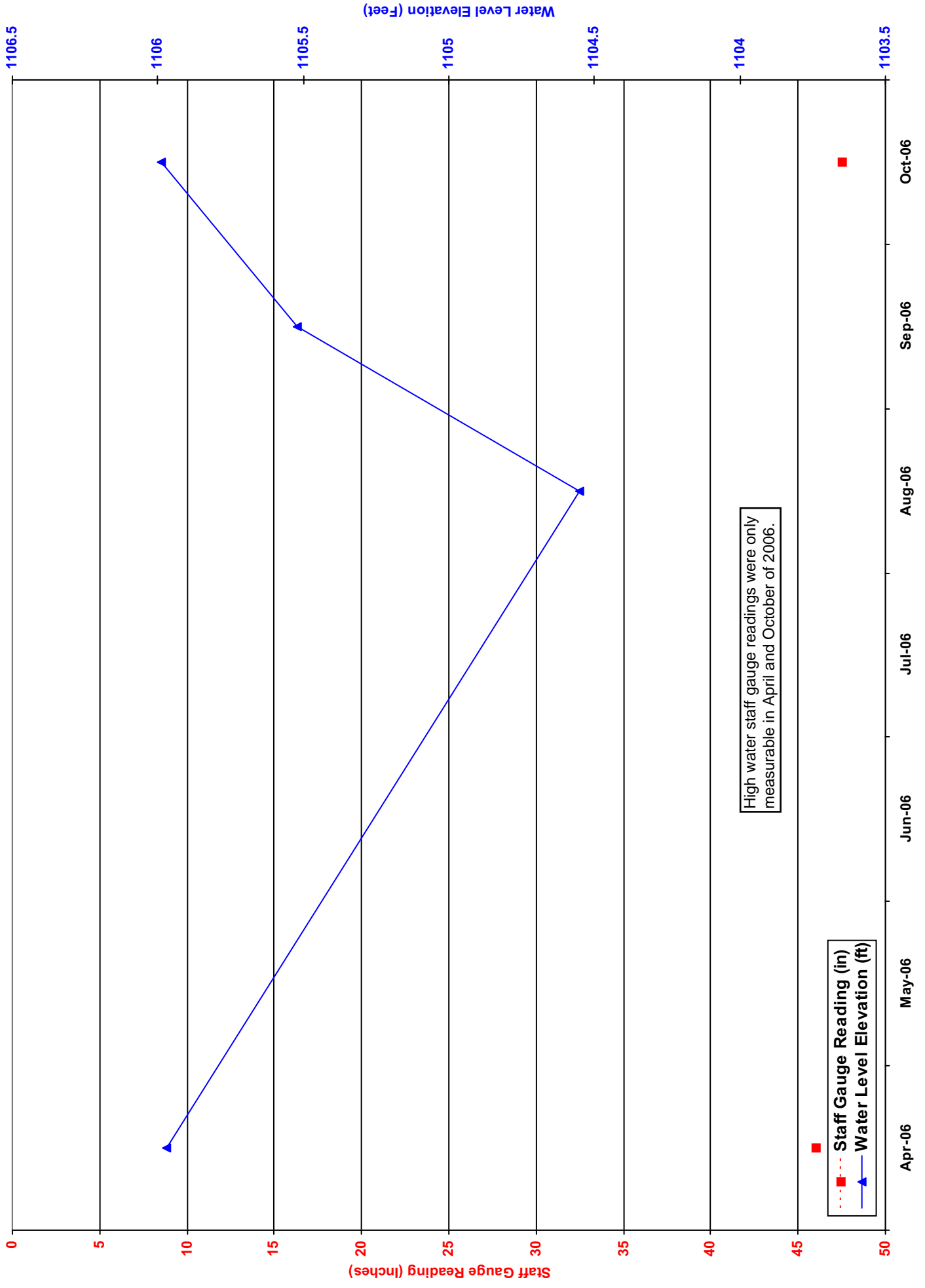
Figure 2 2006 Water Level Elevations for PondDG-13HW
