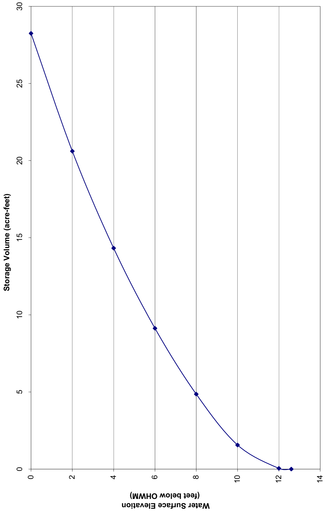
Figure 4 Storage Volume for Pond DG-13
